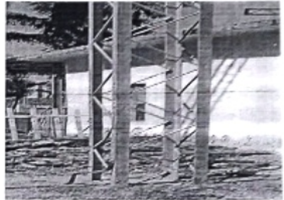
FIG.3 LACING SYSTEM
